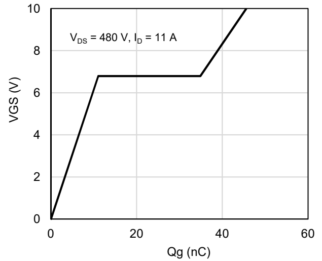
Figure 10: Gate-Charge Characteristics
